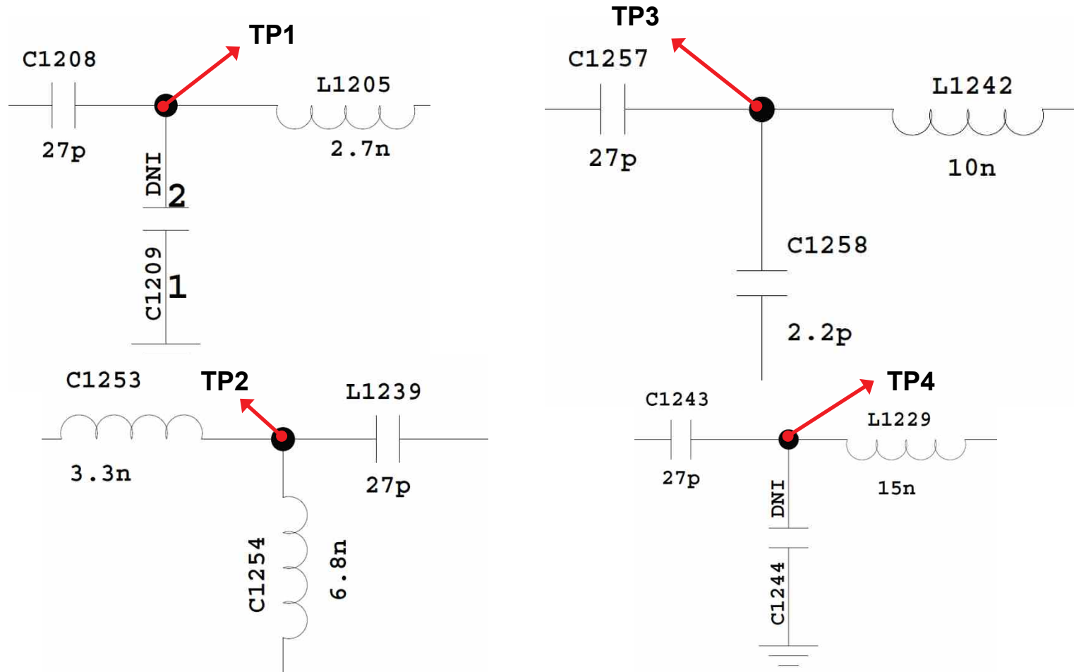
Circuit Diagram
