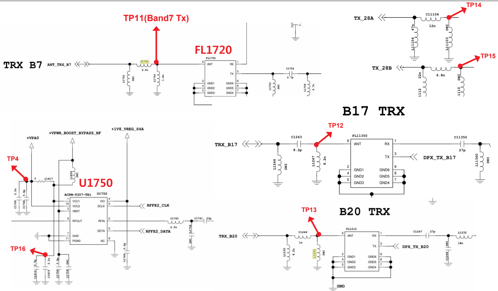
Circuit Diagram
