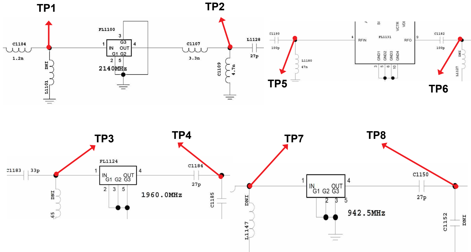
Circuit Diagram
