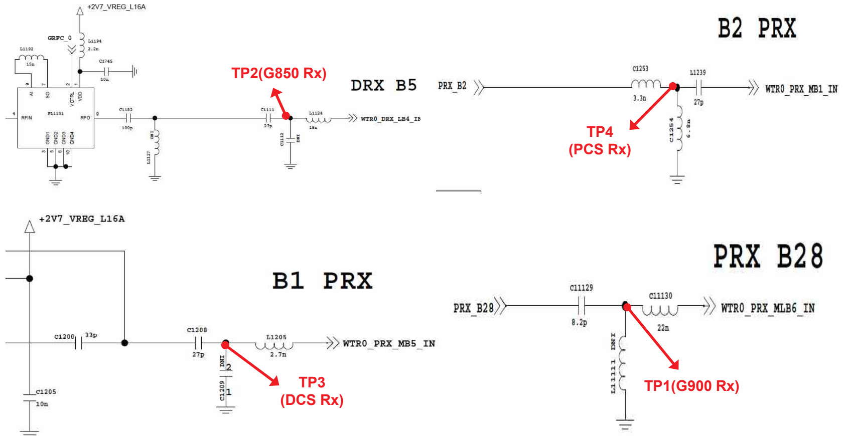
Circuit Diagram
